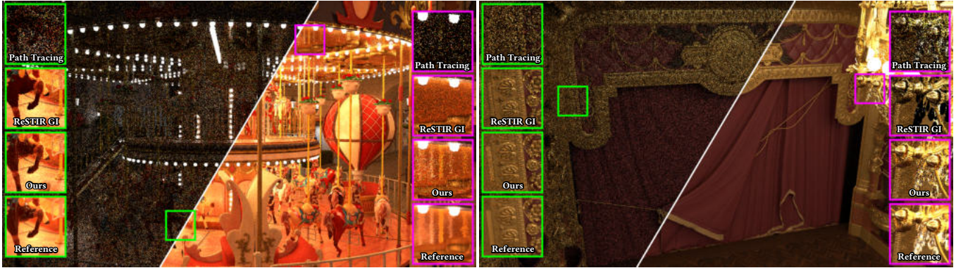
Fig. 1. Our new generalized resampled importance sampling (GRIS) theory extends resampled importance sampling [Talbot 2005] to guarantee convergence even when applied to correlated samples arising from spatiotemporal reuse (i.e., Bitterli et al. [2020]). GRIS allows applying ReSTIR to reuse arbitrary paths, shown with paths of length 10 in the CAROUSEL and PARIS OPERA HOUSE. Main images compare naive path tracing and our new ReSTIR PT in equal time (80 ms at 1920 \times 1080 ). Insets show equal-time path tracing, ReSTIR GI [Ouyang et al. 2021], our ReSTIR PT, plus a converged reference. We significantly improve quality for glossy interreflection, reflections, refractions, and other high-frequency lighting. For CAROUSEL, MAPE errors: path tracing (1.63), ReSTIR GI (0.45), and ReSTIR PT (0.39). Corresponding errors in OPERA HOUSE: 1.28, 0.39, and 0.33. (CAROUSEL ©carousel_world; PARIS OPERA HOUSE courtesy ©GoldSmooth from TurboSquid.)
